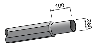
SPIGOT DETAIL
