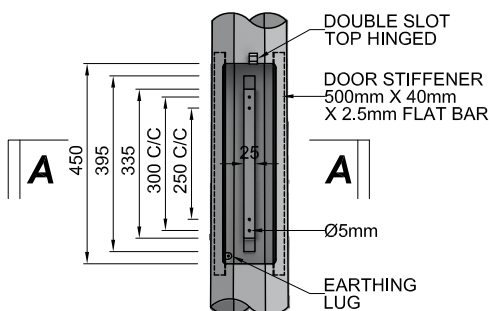
SERVICE DOOR DETAIL
