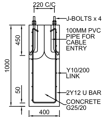
FOOTING DETAIL
