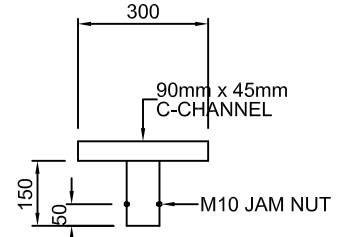
FRONT VIEW HEAD FRAME - 1
