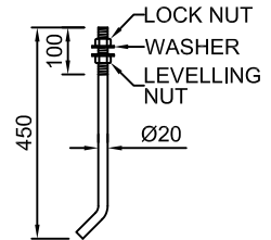
J-BOLT GRADE 4.8
