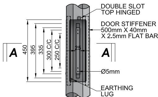
SERVICE DOOR DETAIL
