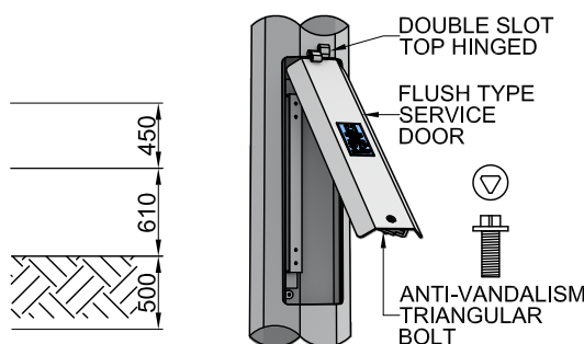
SERVICE DOOR DIAGONAL VIEW
