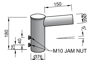
0.15M SINGLE ARM
