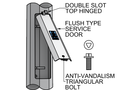
SERVICE DOOR DIAGONAL VIEW
