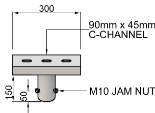
HEAD FRAME - 1
