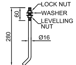
J-BOLT GRADE 4.6
