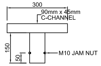
FRONT VIEW HEAD FRAME - 1
