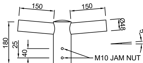
0.15M DOUBLE ARM
