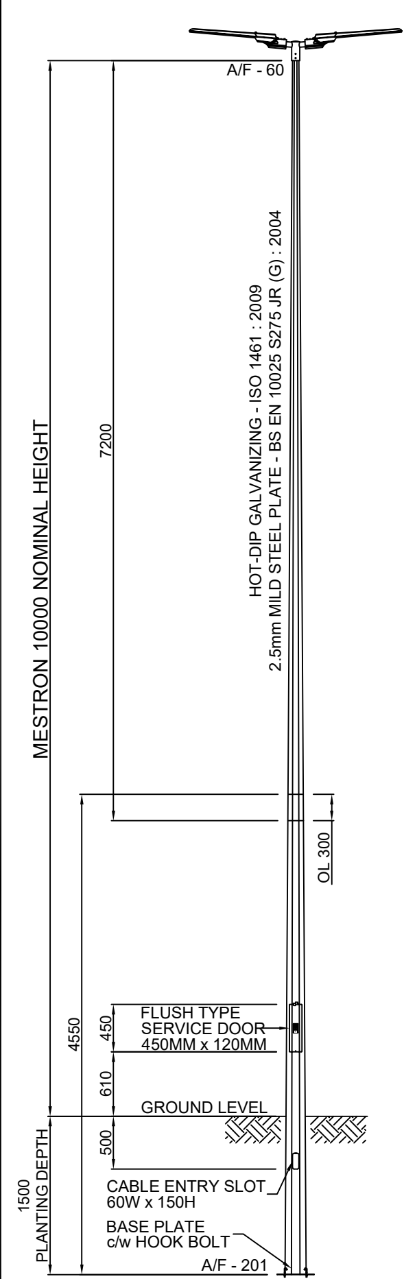
0.15M DOUBLE ARM
