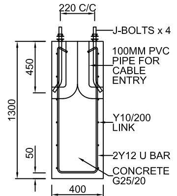
FOOTING DETAIL
