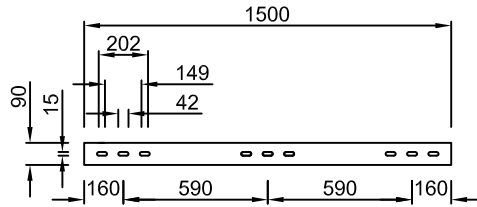
PLAN VIEW HEAD FRAME - 3
