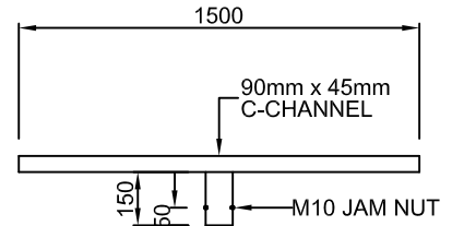
FRONT VIEW HEAD FRAME - 4
