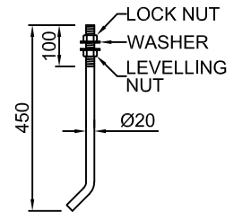
J-BOLT GRADE 4.8
