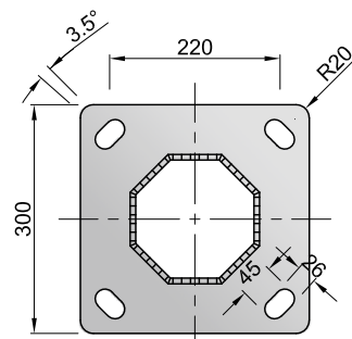
FLANGE PLATE 15mm THK
