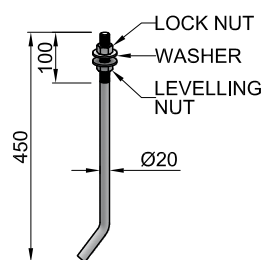
J-BOLT GRADE 4.8
