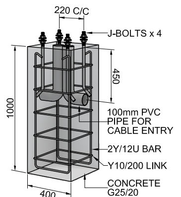
FOOTING DETAIL
