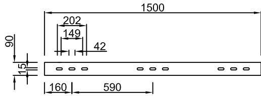
PLAN VIEW HEAD FRAME - 3
