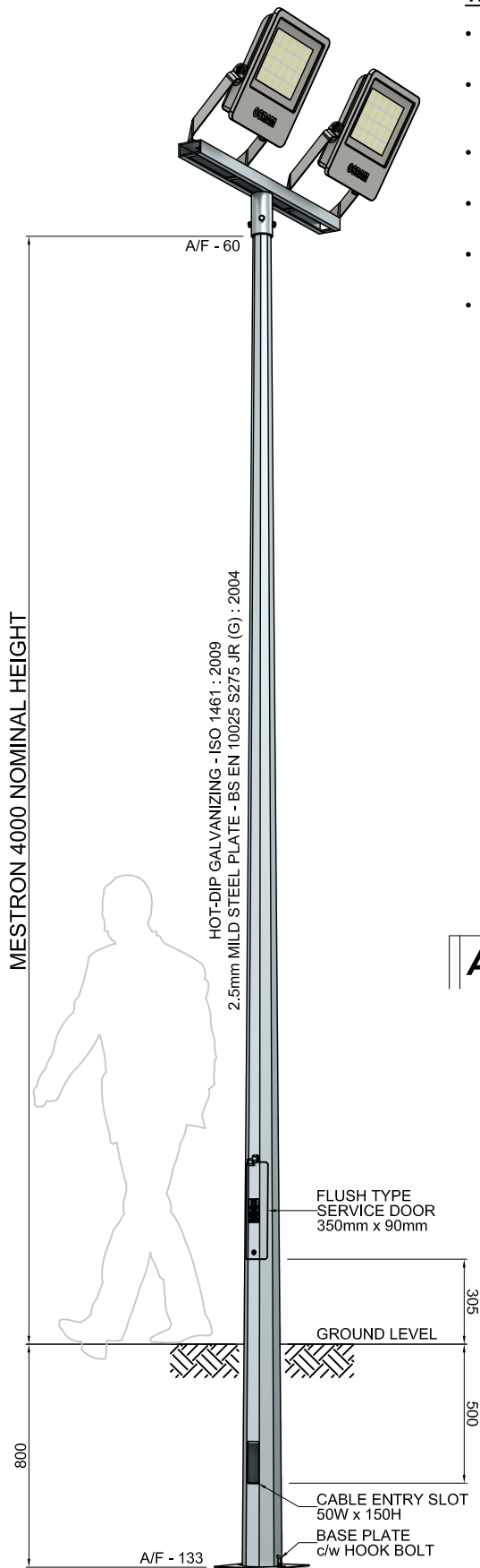
HEAD FRAME - 2
