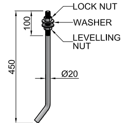
J-BOLT GRADE 4.8
