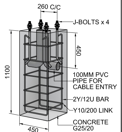
FOOTING DETAIL
