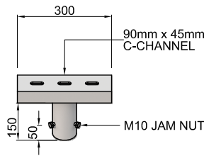
HEAD FRAME - 1
