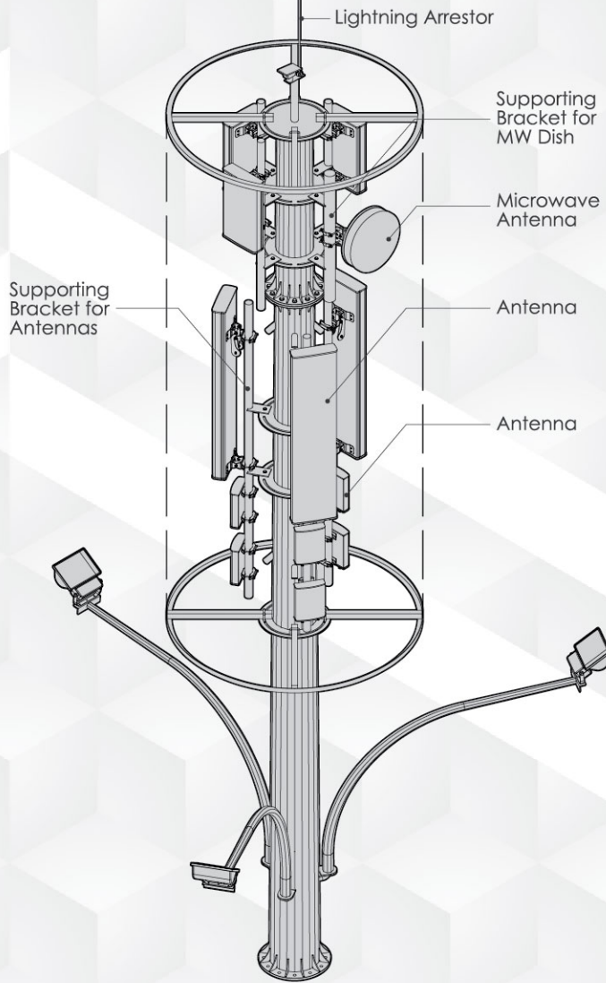
Mounting Brackets - 3D Isometric View
