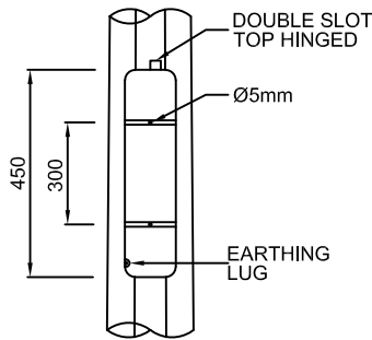
SERVICE DOOR DETAIL
