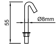
HOOK BOLT
