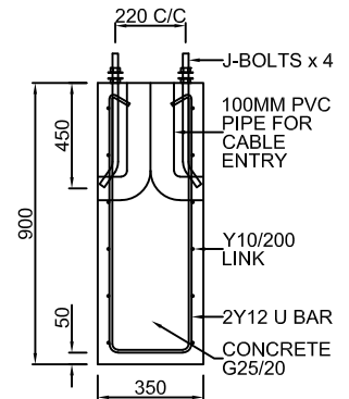
FOOTING DETAIL
