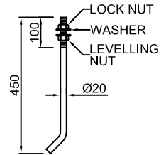
J-BOLT GRADE 4.6
