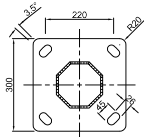
FLANGE PLATE 12mm THK
