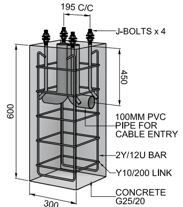
FOOTING DETAIL
