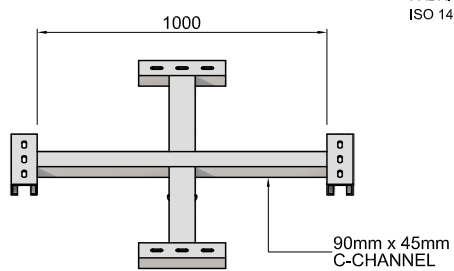
HEAD FRAME - 4
