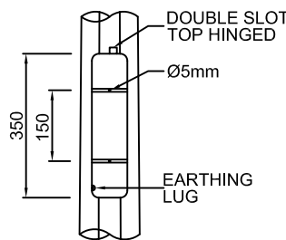
SERVICE DOOR DETAIL
