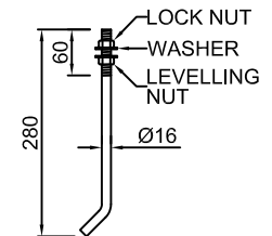
J-BOLT GRADE 4.6
