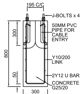
FOOTING DETAIL
