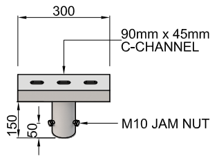
HEAD FRAME - 1
