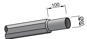
SPIGOT DETAIL
