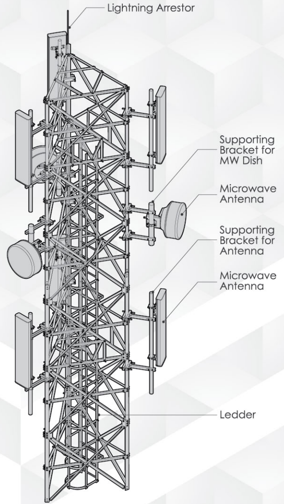
Top Section - 3D Isometric View
