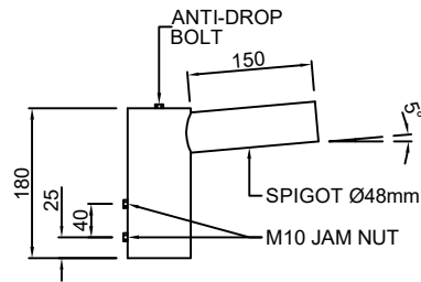
SIDE VIEW 0.15M SINGLE ARM
