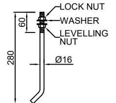
J-BOLT GRADE 4.8
