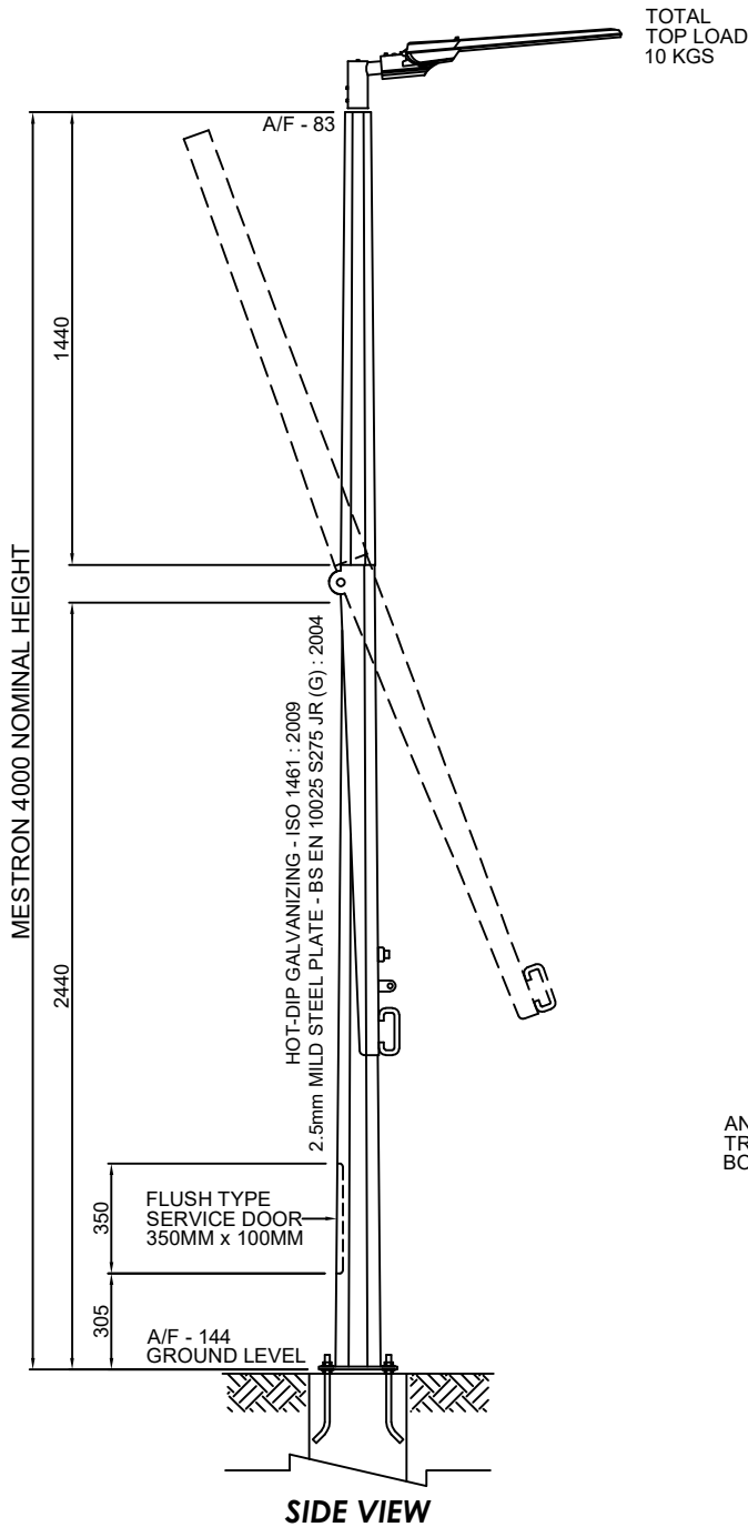
SIDE VIEW 0.15M SINGLE ARM
