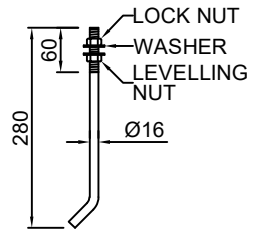
J-BOLT GRADE 4.8
