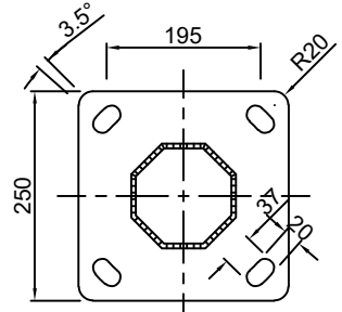
FLANGE PLATE
