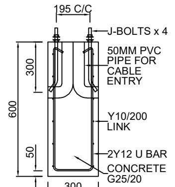
FOOTING DETAIL
