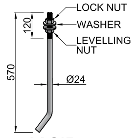
J-BOLT GRADE 4.8
