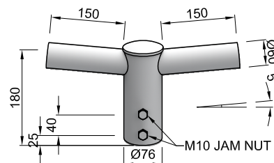
0.15M DOUBLE ARM
