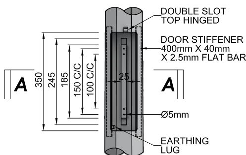
SERVICE DOOR DETAIL
