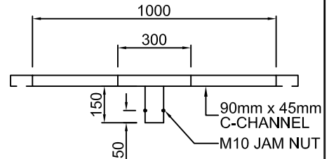
FRONT VIEW HEAD FRAME - 4
