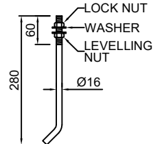
J-BOLT GRADE 4.8
