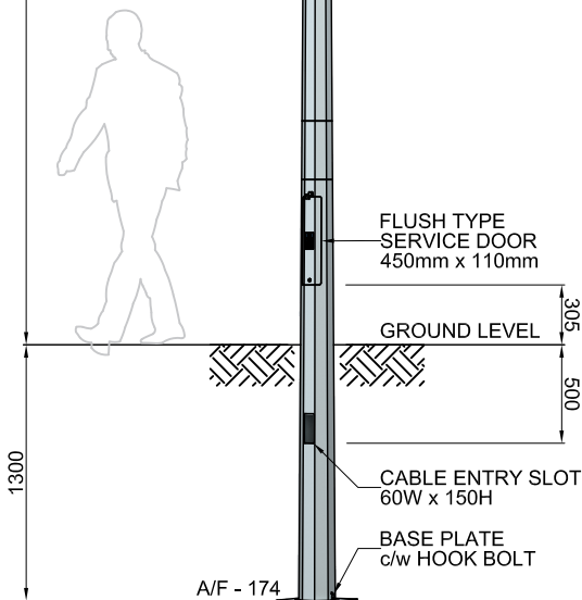
SERVICE DOOR DETAIL
