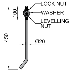
J-BOLT GRADE 4.8
