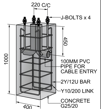
FOOTING DETAIL
