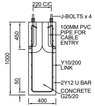
FOOTING DETAIL
